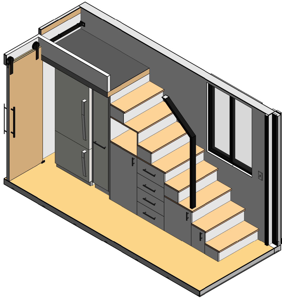
2 CABINETRY 3D 02
