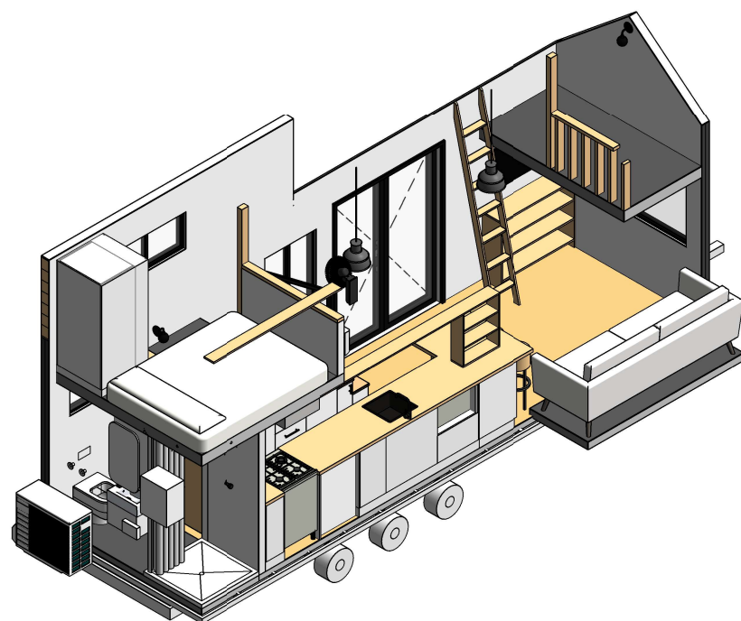
3 3D 03
