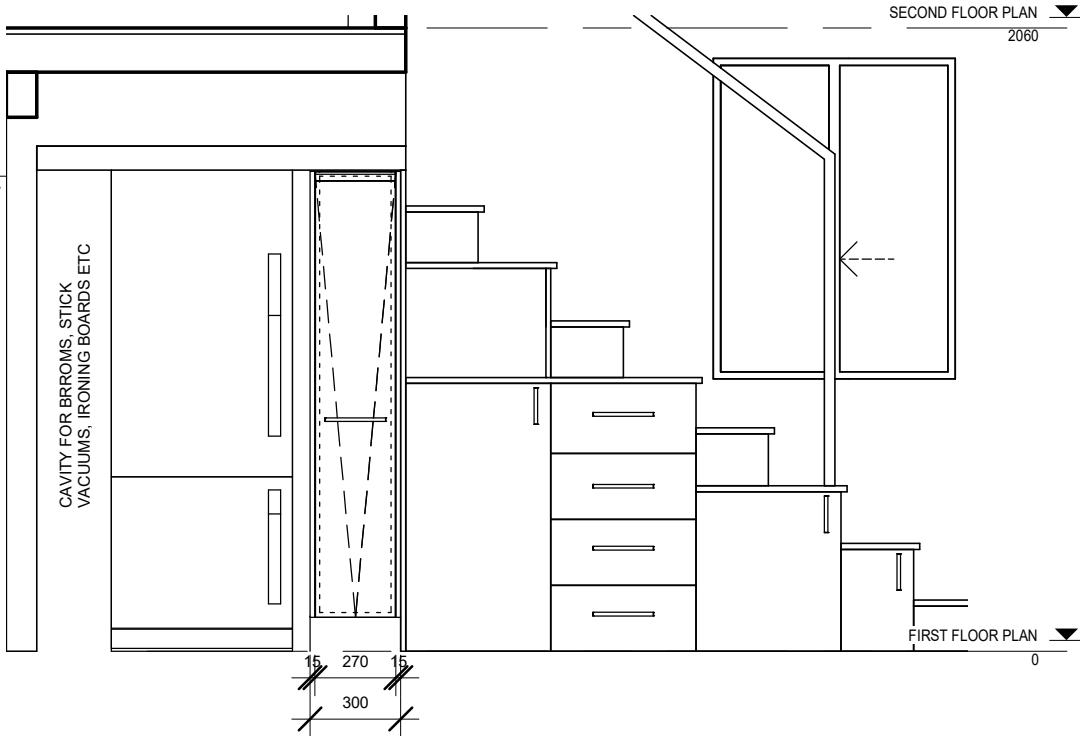
2 CABINETRY ELEVATION 01 07 1 : 25
