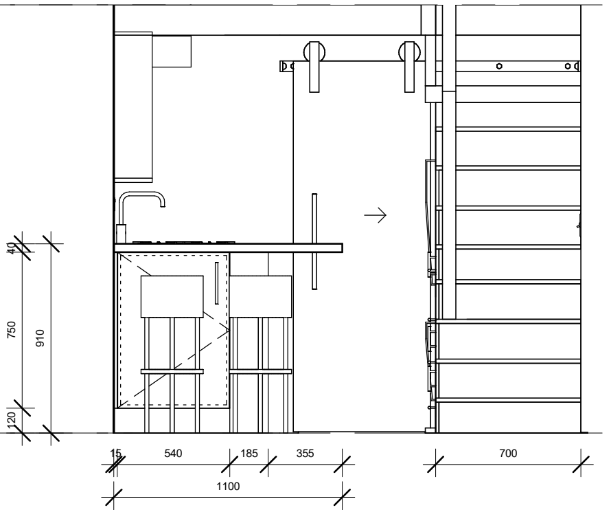
4 CABINETRY ELEVATION 03 07 1 : 25
