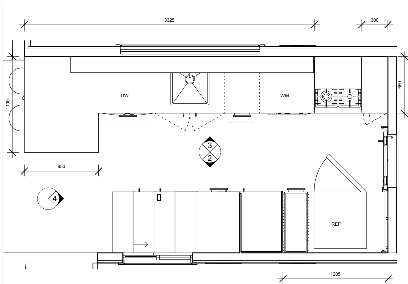
1 KITCHEN CABINETRY 1 : 25
